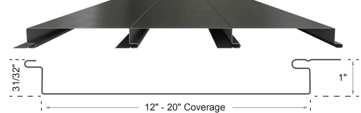
Flush Wall Concealed Fasteners 24ga Wall Panel
