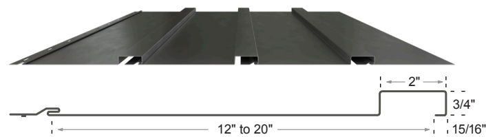
Board and Batten Concealed Fasteners 24ga Wall Panel
